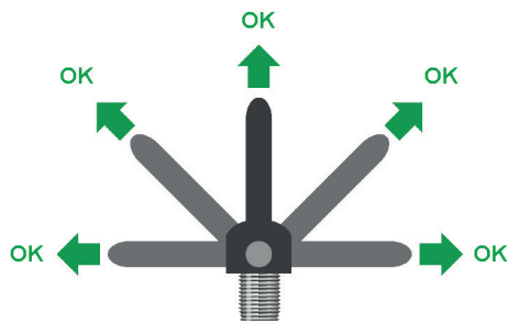
Swivel Hoist Ring Full load rating at any angle
