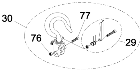
Cast Latch Kit for 1/2 -5t hoist with Serial # \geq 12G1562-09
