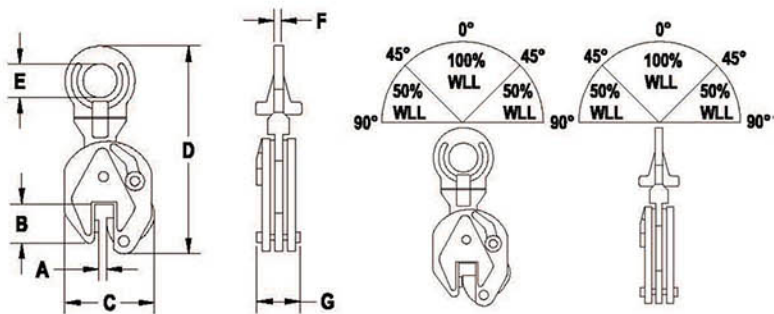
PCUA SERIES SPECIFICATIONS AND DIMENSIONS (inches)
