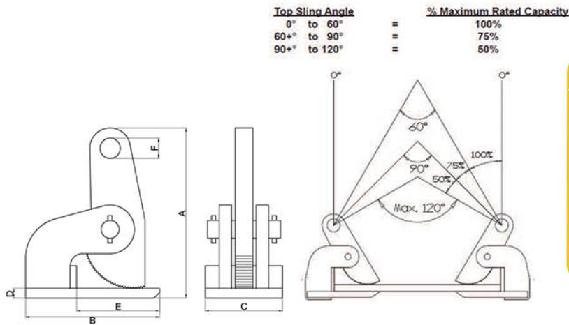
PCH SERIES SPECIFICATIONS AND DIMENSIONS (inches)
