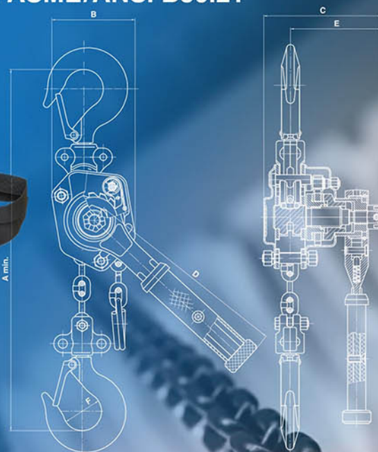
LZ Series Specifications and Dimensions (inches and pounds)
